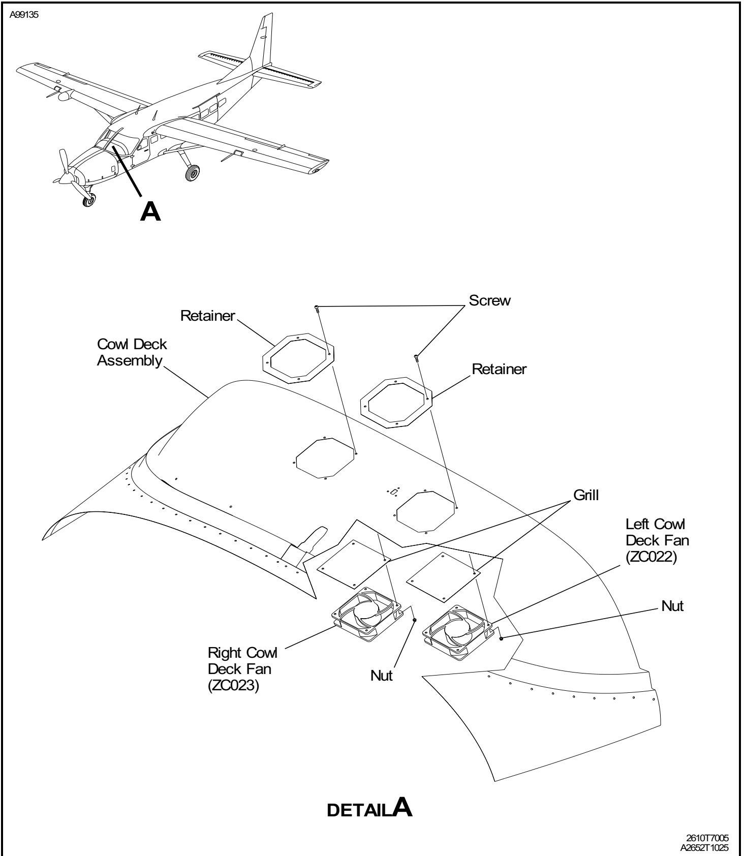
Figure 401 : Sheet 1 : Cowl Deck Cooling Fan Installation
